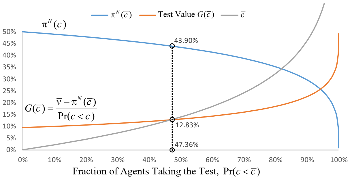
Figure 4: Example of equilibrium construction when c is distributed according to an exponential distribution with mean 20%. The remaining parameters are the same as in Figure 1. The test value is the RHS of (14); an equilibrium is found when this value is equal to \bar{c} . In this example, the equilibrium \pi^N = 43.90\% and \bar{c} = 12.83\% . The 47.36% of agents who take the test receive an average price of \pi^N + G(\bar{c}) = 56.73\% .
